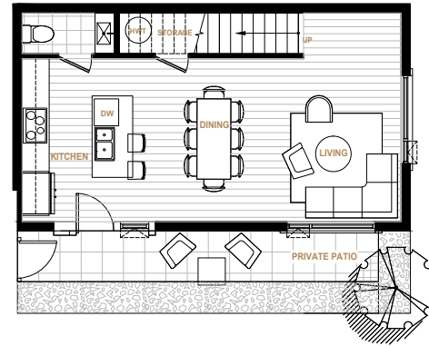
MAIN LEVEL
