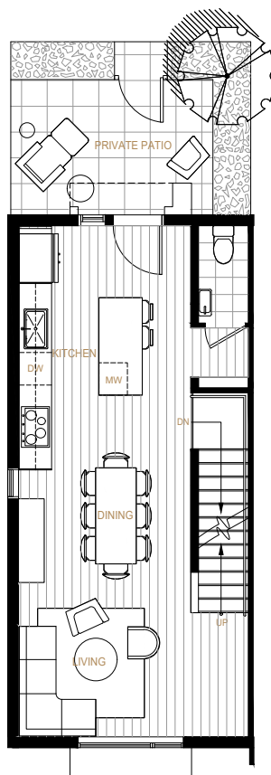
MAIN LEVEL
