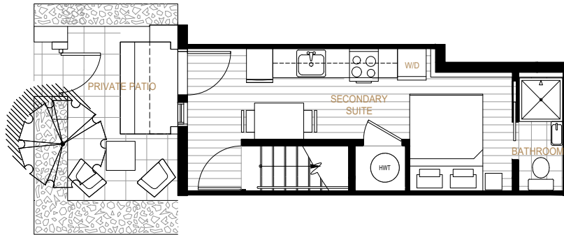
GROUND LEVEL
