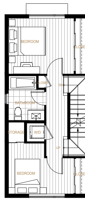
SECOND LEVEL
