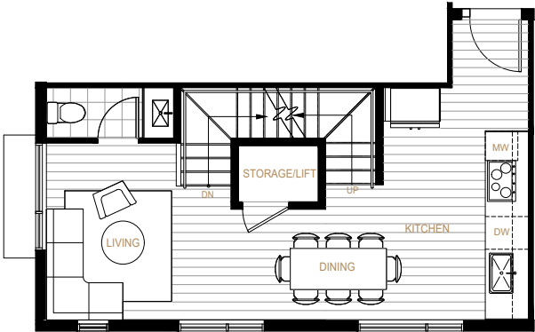
MAIN LEVEL
