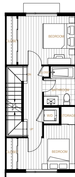
SECOND LEVEL
