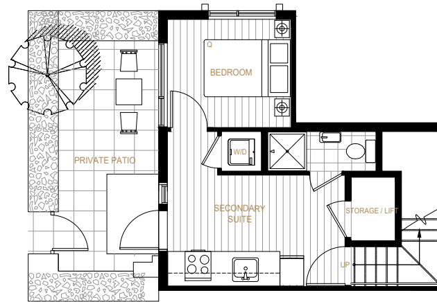
GROUND LEVEL
