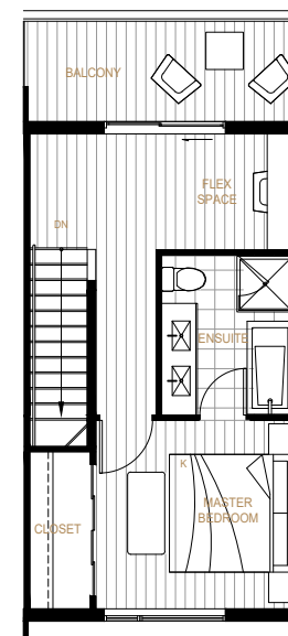
UPPER LEVEL
