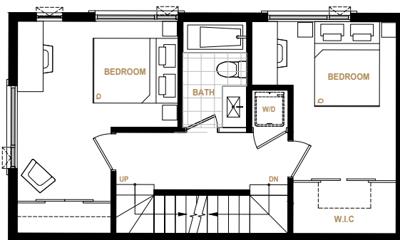
SECOND LEVEL
