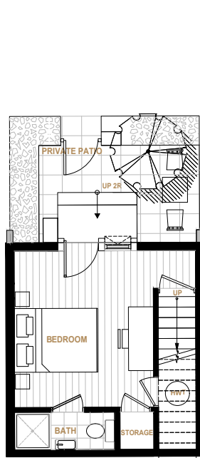
GROUND LEVEL
