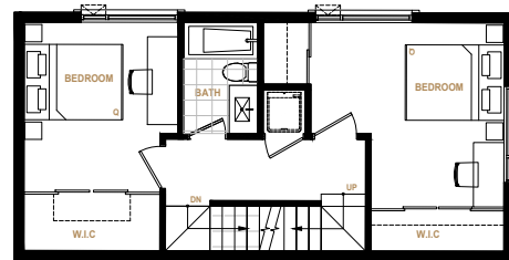
SECOND LEVEL
