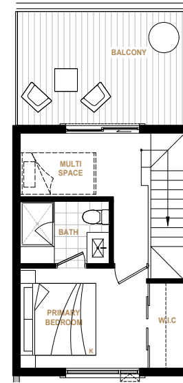
UPPER LEVEL
