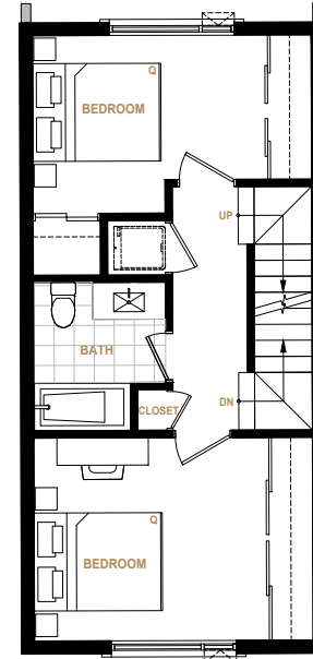
SECOND LEVEL
