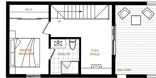
UPPER LEVEL
