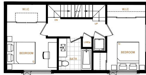
SECOND LEVEL
