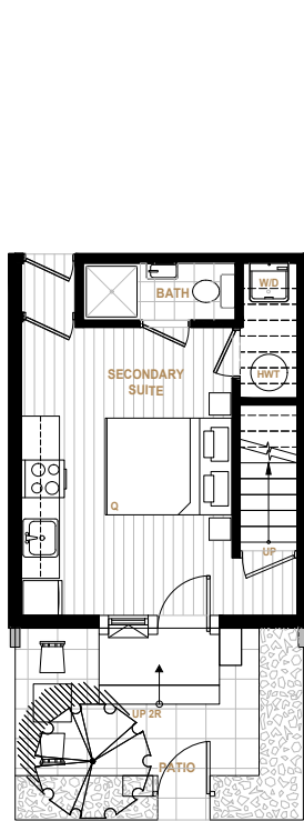
GROUND LEVEL
