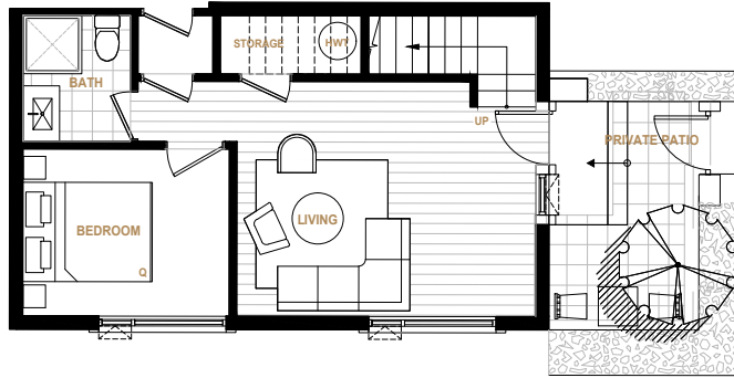
GROUND LEVEL
