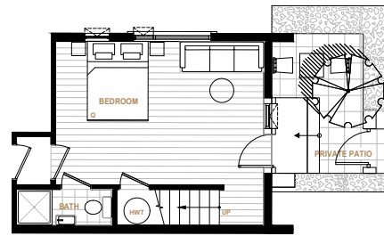
GROUND LEVEL
